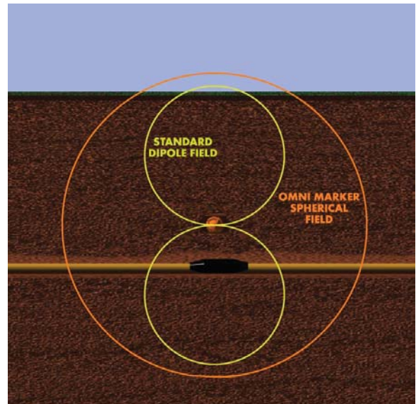
Omni Marker spherical field compared to the standard 3M Ball Marker dipole field.
